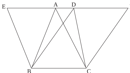
Figure 1 Proposition I.37 of Euclid's Elements .
